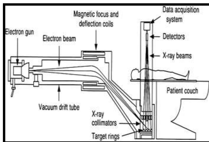
Figure 7. Fifth Generation of Ct [1]
