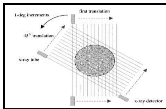
Figure 3. First Generation Computed Tomography
