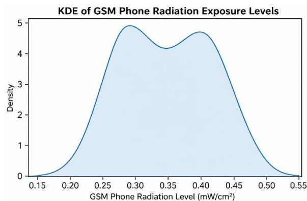
Figure 2. KDE of GSM Phone Radiation Exposure Levels
