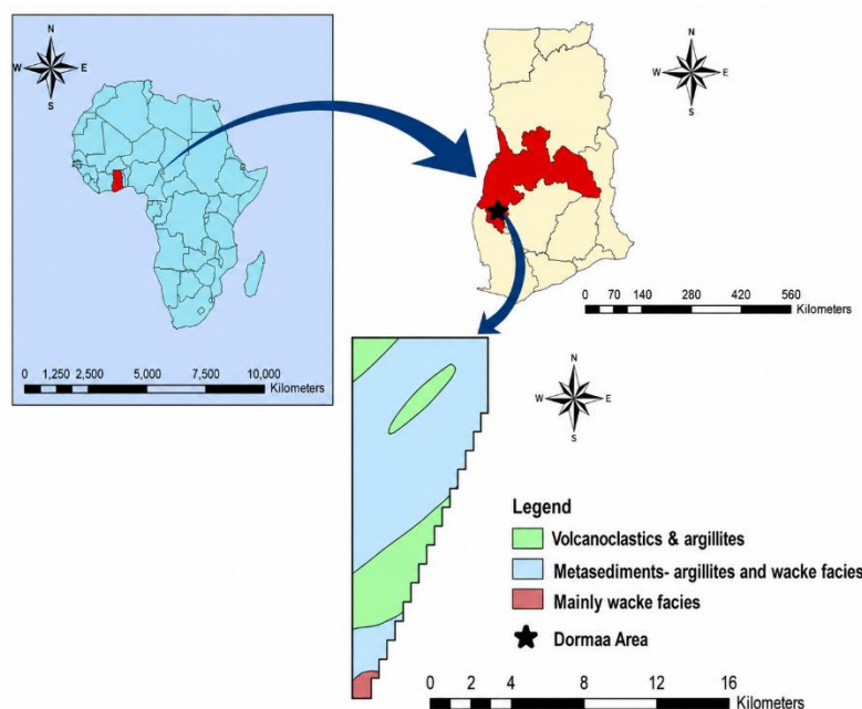
Figure 1. Location and Geology of the Study Area
