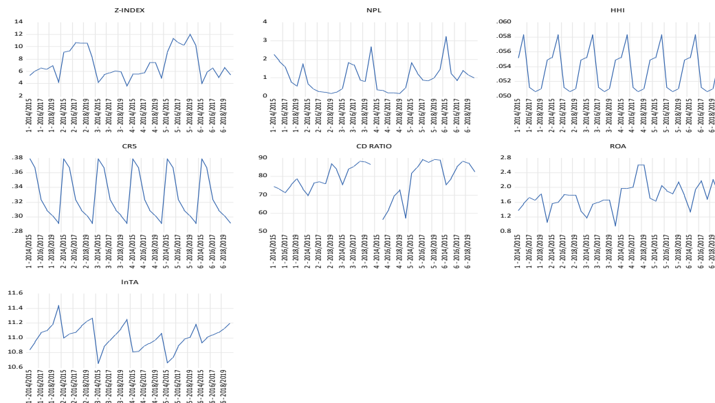
Figure 2: Graphical presentation of all variables
