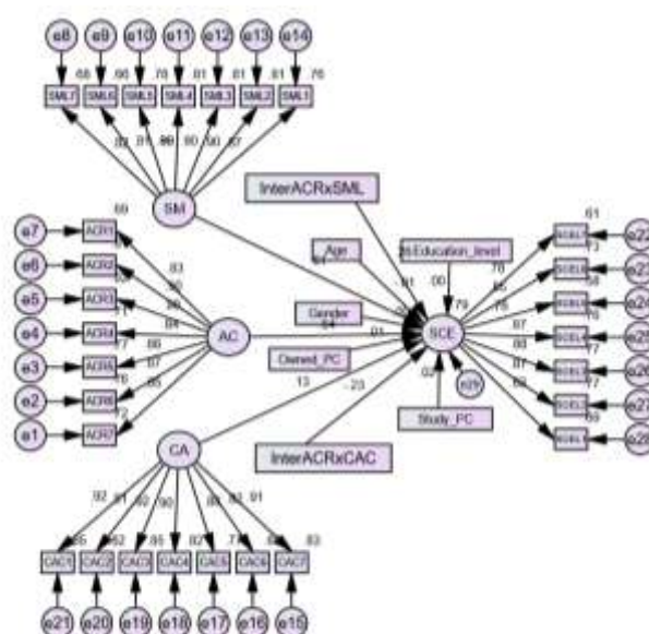
Figure 3: Structural Equation Model
