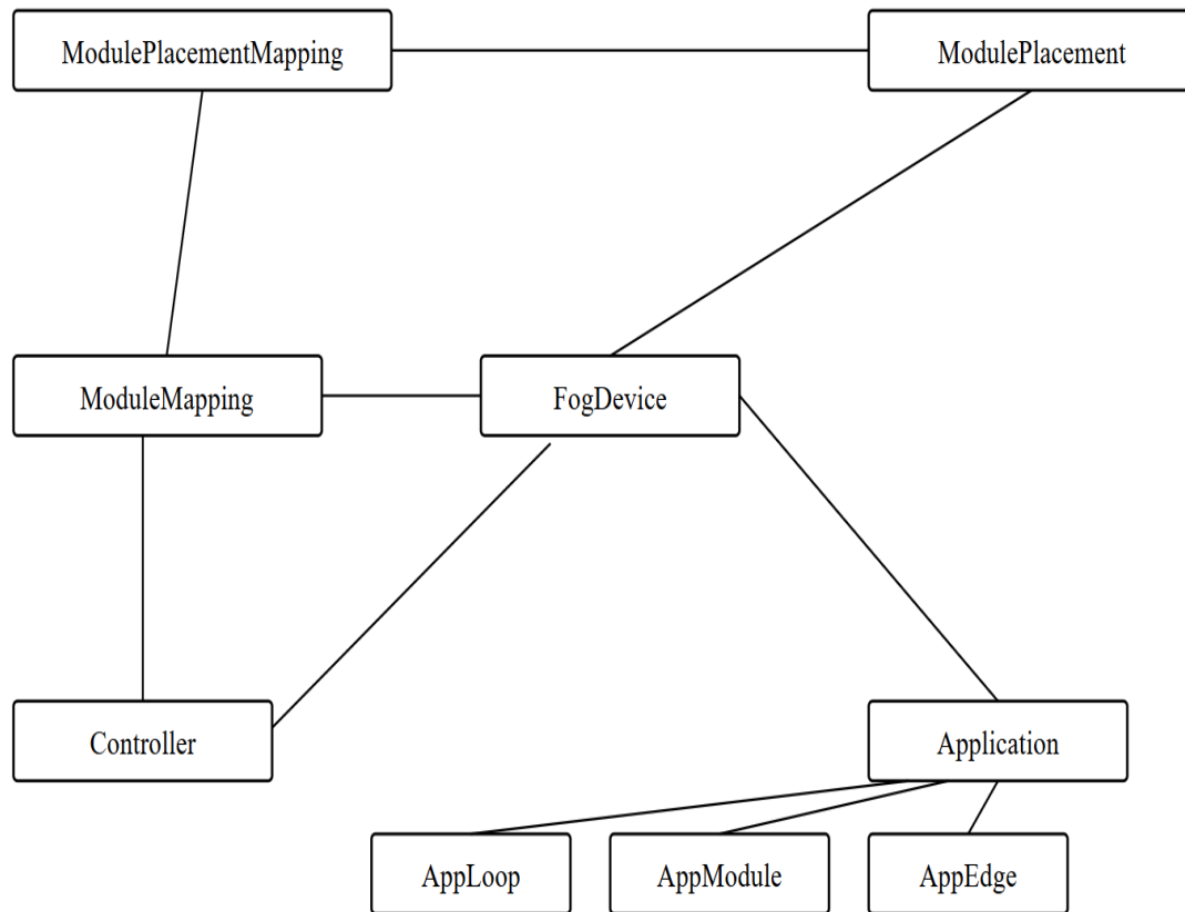
Figure 7. Fog Devices and Modules Placement in Fog Simulation
