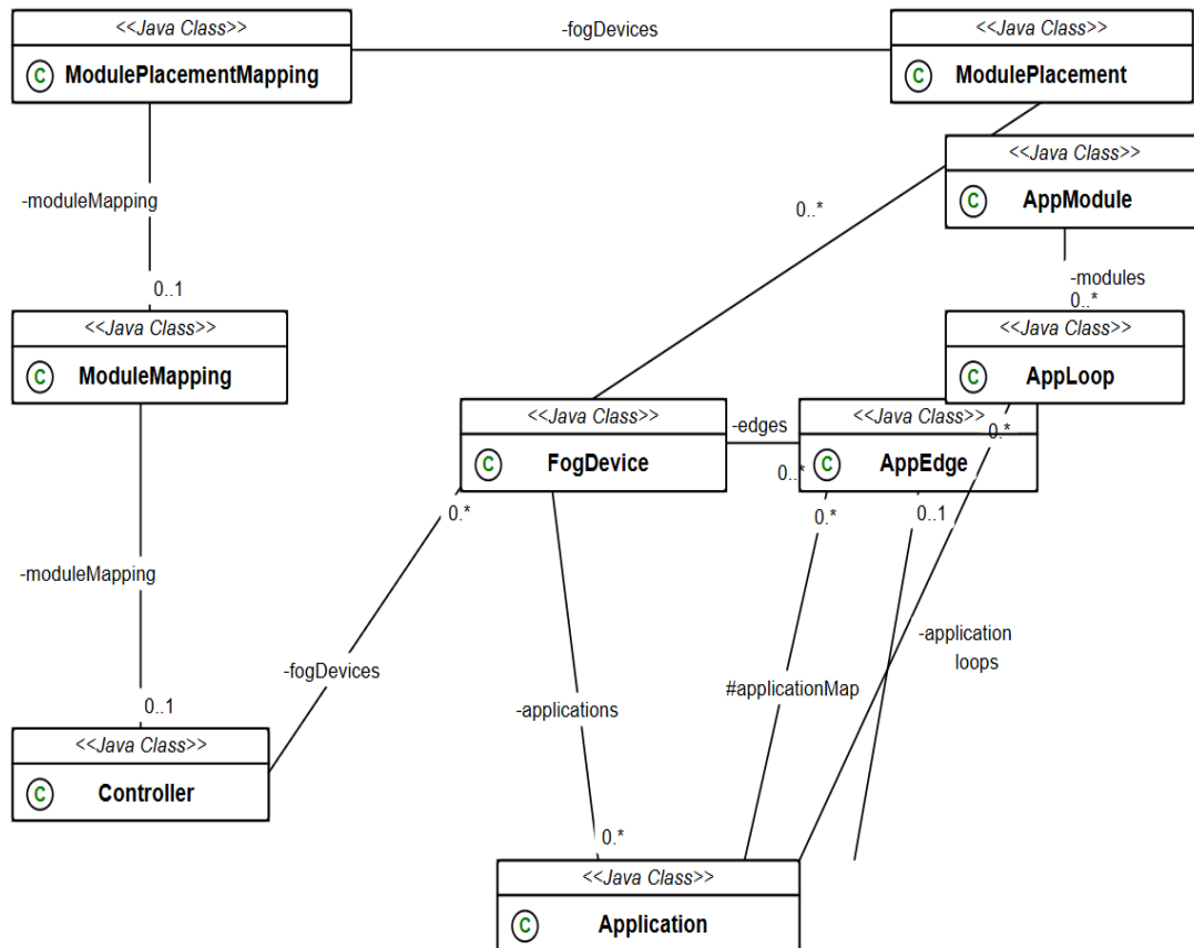
Figure 4. Modules and Classes in iFogSim
