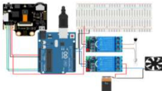
Figure 12: Circuit Diagram for Home Automation Using AI Tools
