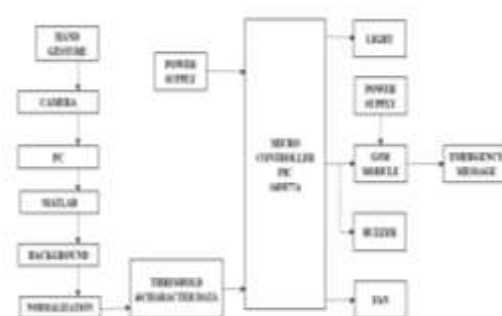
Figure 1: Microcontroller Block Layout
