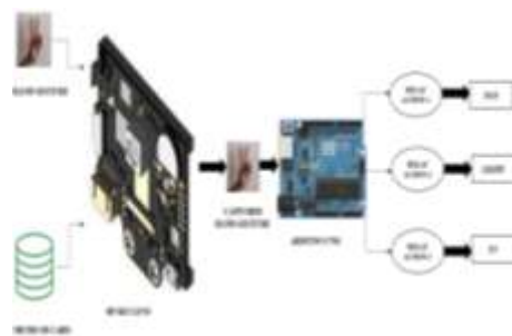
Figure 6: Block Diagram of Home Automation Using AI Tools
