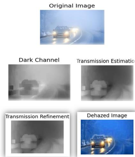
Figure 4. Result of One Frame Processing
