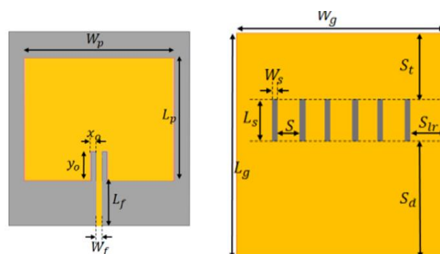
Figure 4. Patch Antenna Top Plane and Bottom Plane with Defected Ground Structure
