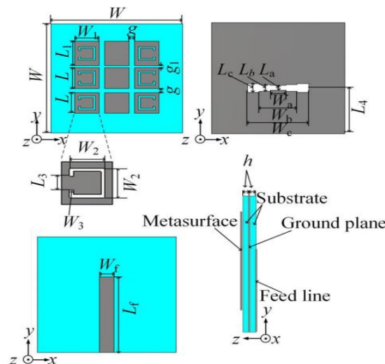
Figure 2. Configuration of Metasurface Antenna [41]
