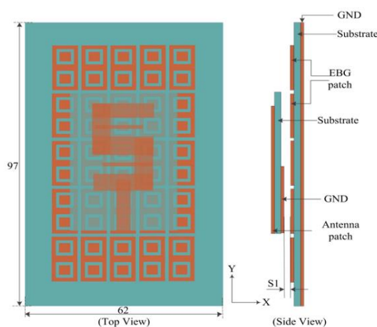
Figure 3. Monopole Antenna with Electromagnetic Bandgap Structure
