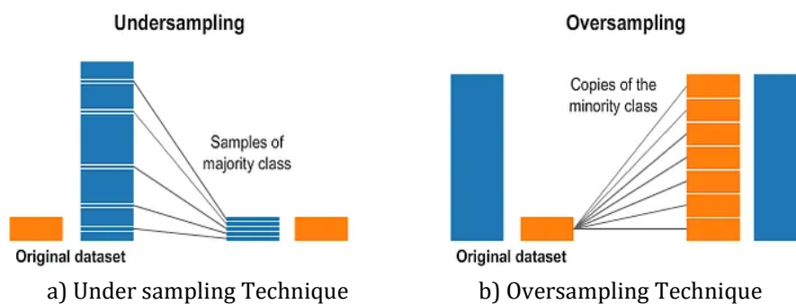
Figure 1. Resampling Methods
