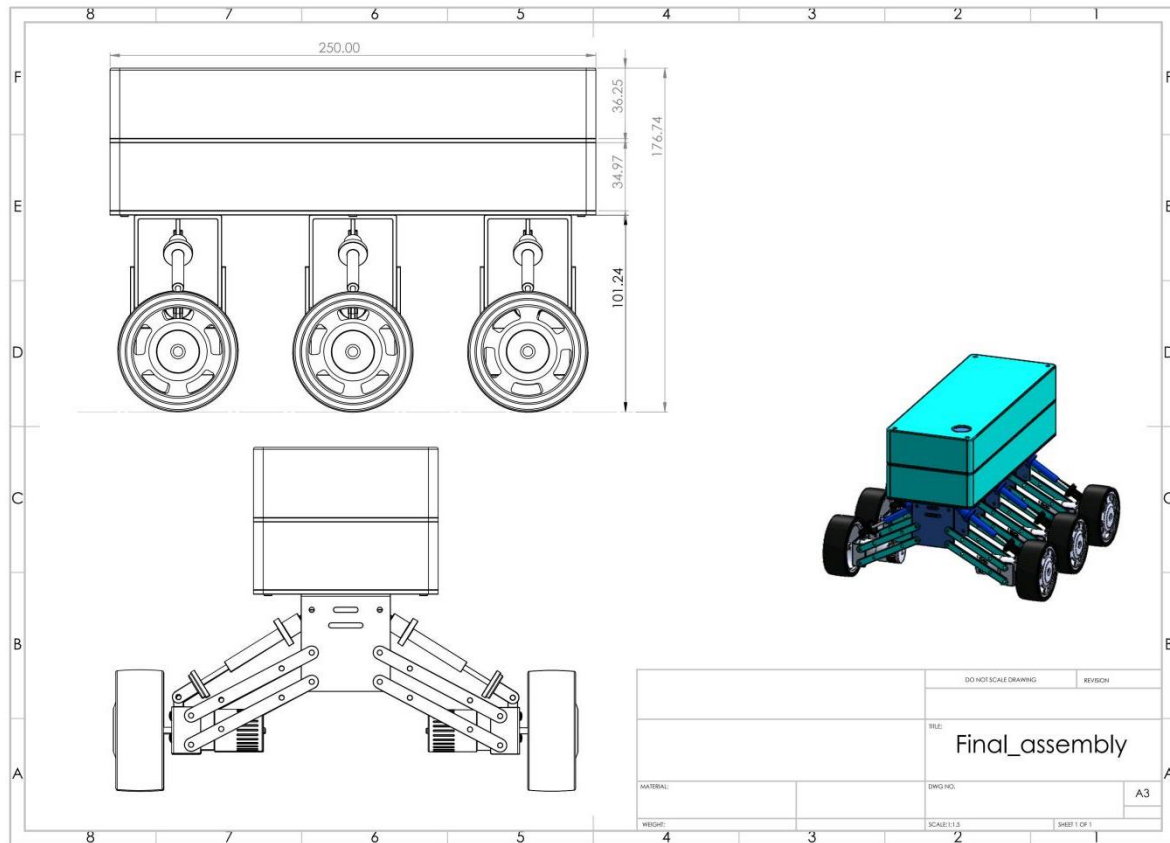
Figure 10. Final Assembly
