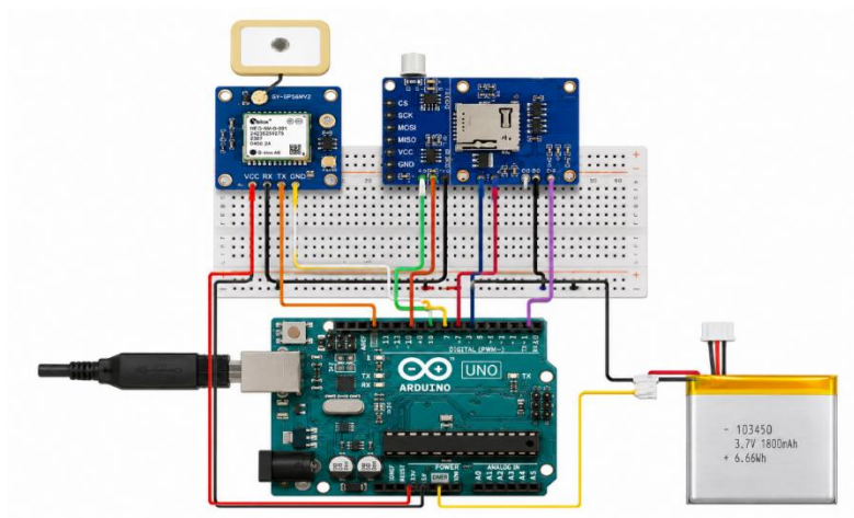
Figure 5. Component Connection Circuit
