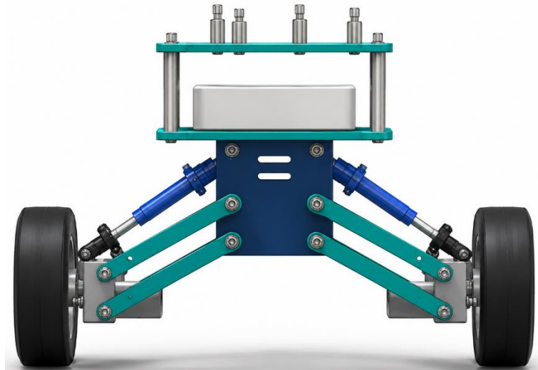
Figure 12. Front View
