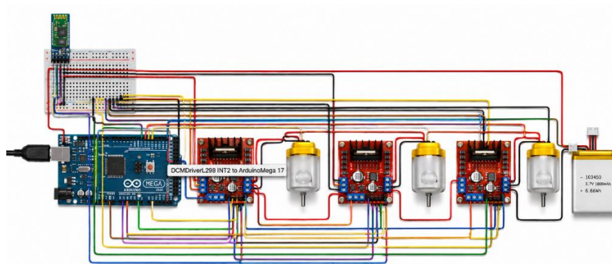
Figure 6. Motor Controller Circuit
