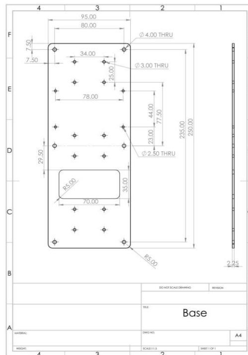
Figure 7. First Base Plate
