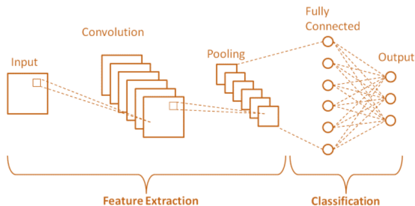
Figure 2. Basic Architecture of CNN
