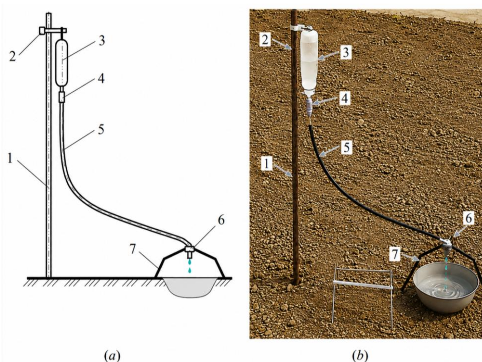
Figure 1. Drip Device: General View of the A-Device; B-Picture of the Device
